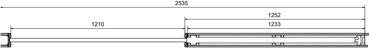
SECTIONAL VIEW 1:15 THE WALL FRAME; SLIDING DOOR ELEMENT, PLASTERBOARDS, DOOR AND FRAMES
