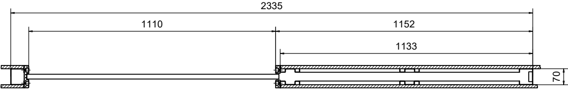
SECTIONAL VIEW 1:15 THE WALL FRAME; SLIDING DOOR ELEMENT, PLASTERBOARDS, DOOR AND FRAMES
