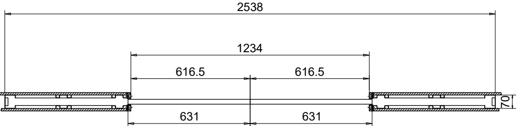
SECTIONAL VIEW 1:25 THE WALL FRAME; SLIDING DOOR ELEMENT, PLASTERBOARDS, DOORS AND FRAMES
