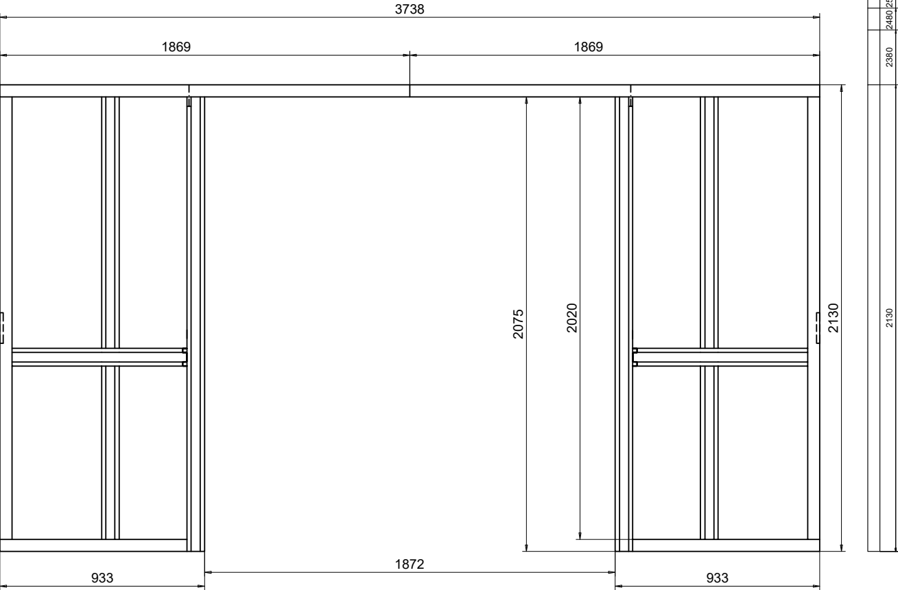
FRONT VIEW 1:25 SLIDING DOOR ELEMENT LI014DD
