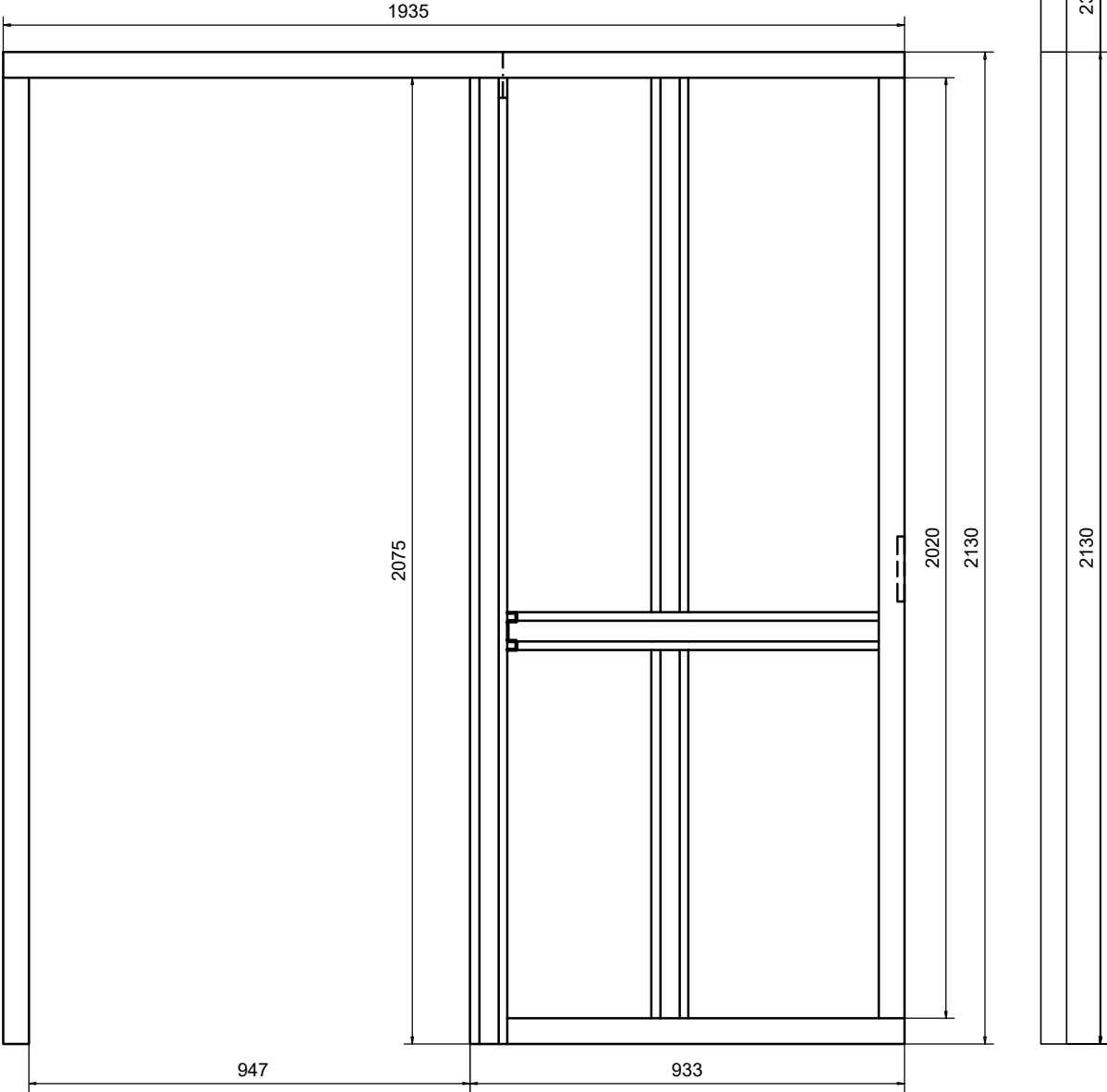
FRONT VIEW 1:15 SLIDING DOOR ELEMENT LI09
