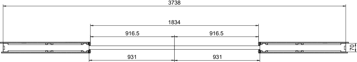
SECTIONAL VIEW 1:25 THE WALL FRAME; SLIDING DOOR ELEMENT, PLASTERBOARDS, DOORS AND FRAMES
