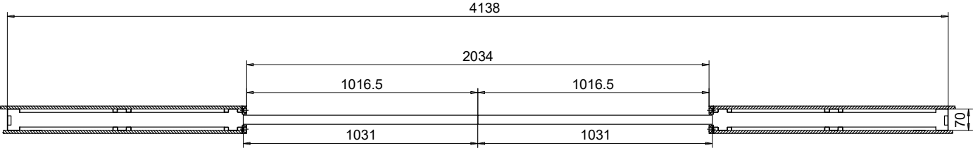
SECTIONAL VIEW 1:25 THE WALL FRAME; SLIDING DOOR ELEMENT, PLASTERBOARDS, DOORS AND FRAMES
