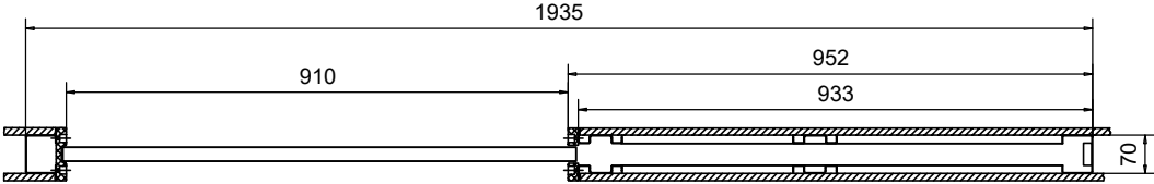
FRONT VIEW 1:15 SLIDING DOOR ELEMENT LI09
