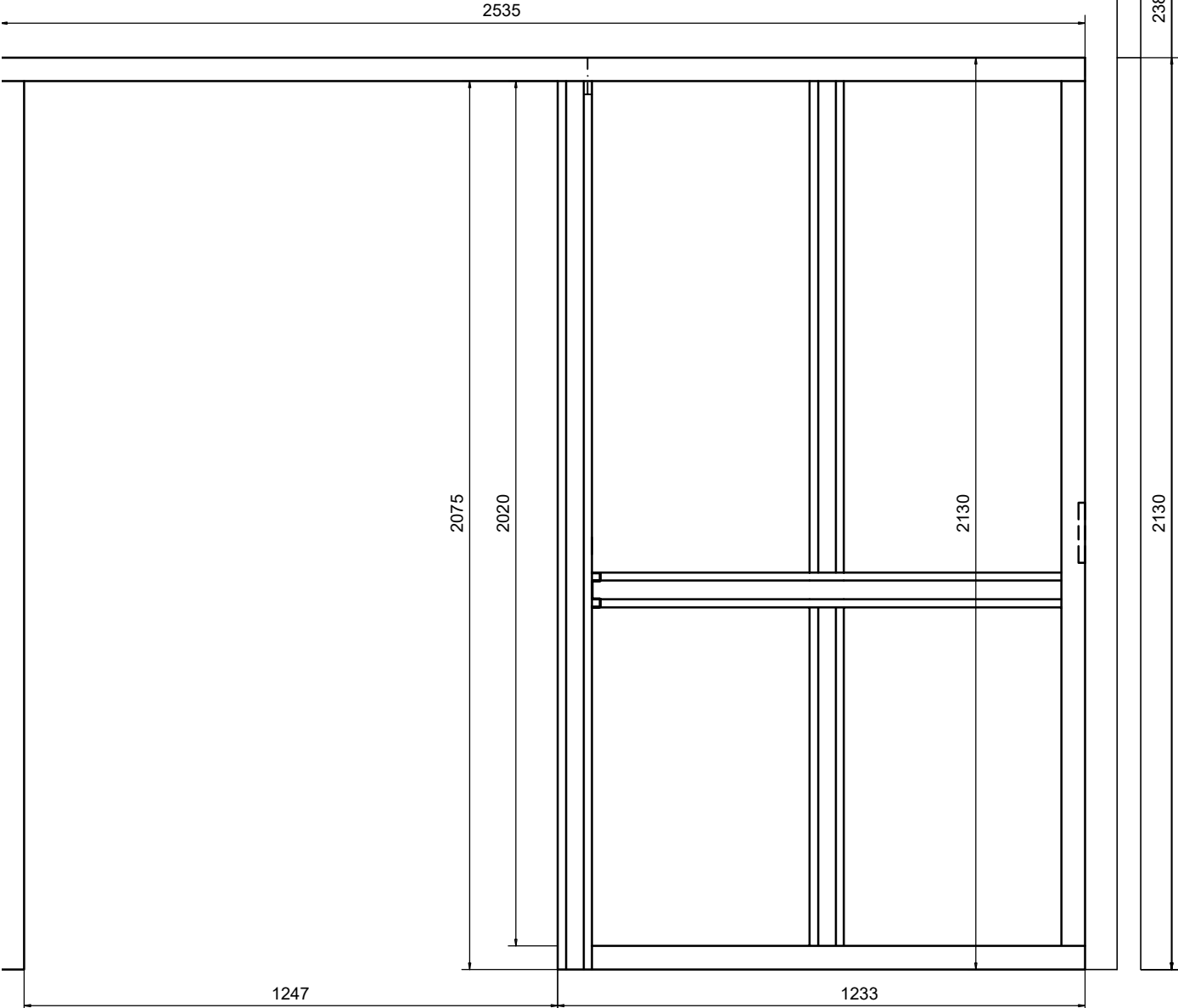
FRONT VIEW 1:15 SLIDING DOOR ELEMENT LI012
