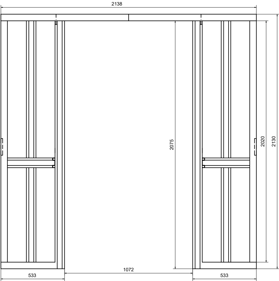
FRONT VIEW 1:15 SLIDING DOOR ELEMENT LI010DD
